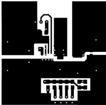
Figure 6c. Top-Side Copper
